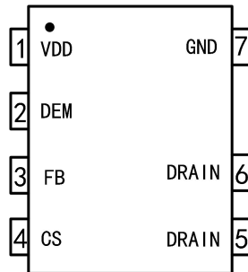
SOP7 Package
