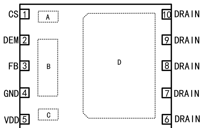
DFN6X5-10L Package
