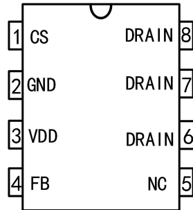
Pin Configuration: G1565AP Series
