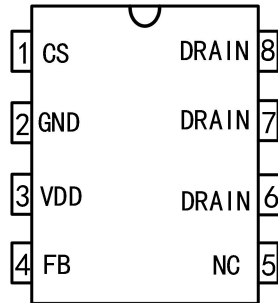
Pin Configuration: G1587AP Series
