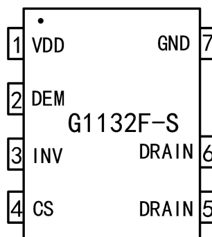
SOP7 Package
