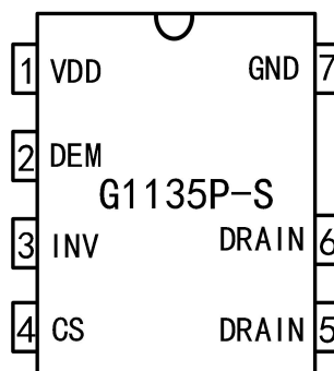
DIP7 Package
