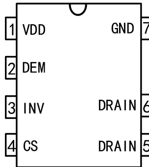
DIP7 Package
