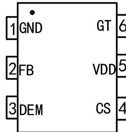
SOT23-6 Package
