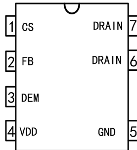
DIP8 Package
