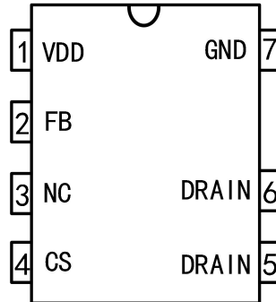
Pin Configuration: G1589P Series
